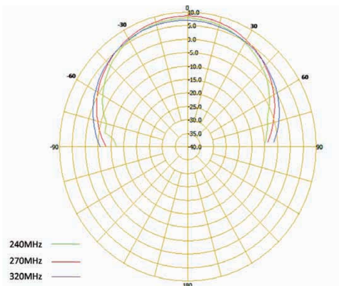
Radiation Pattern
